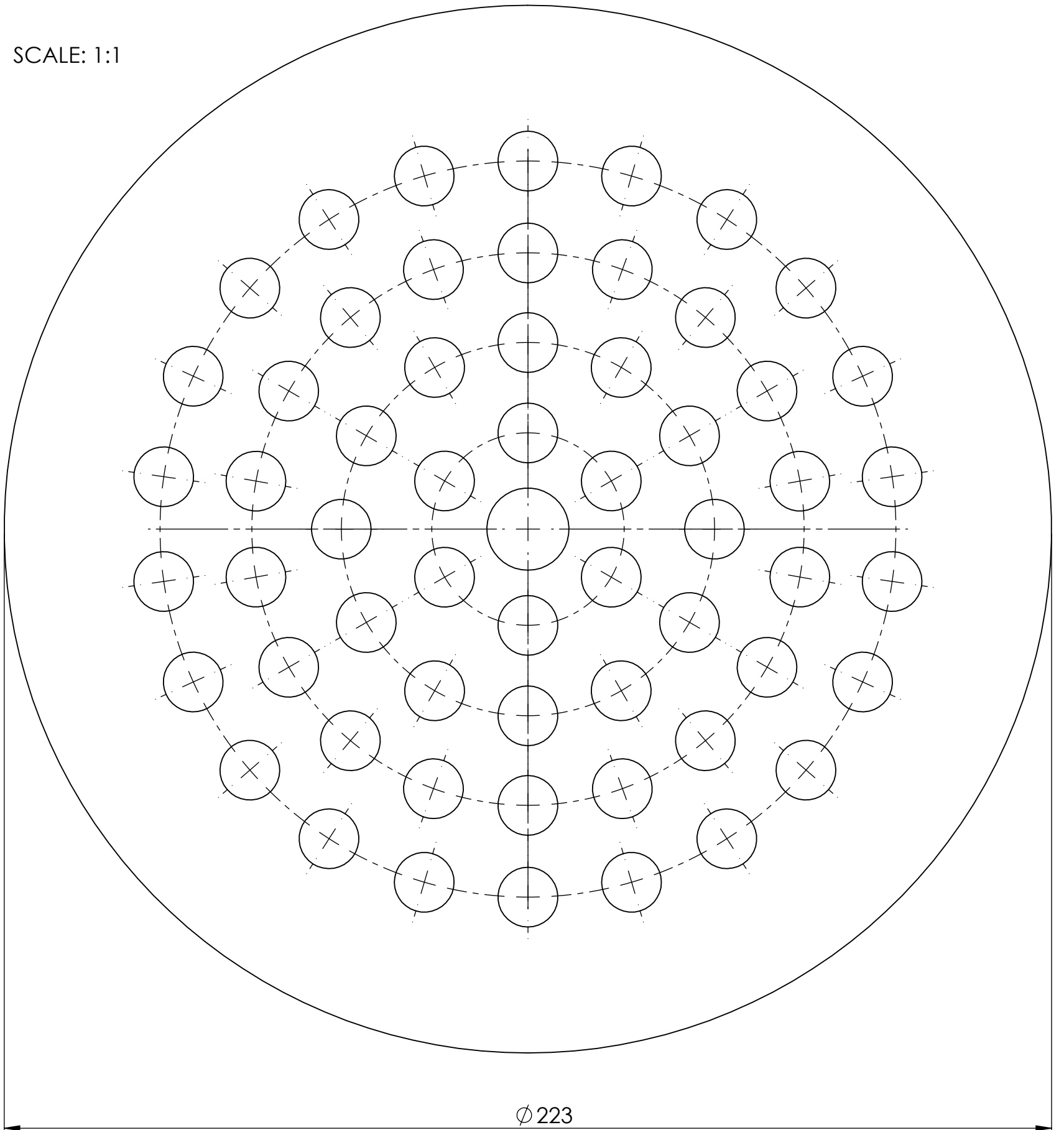
AME #176: 8" Diameter Boiler. Tube plate Flat Pattern. Leave out the center hole for the top tube plate.
